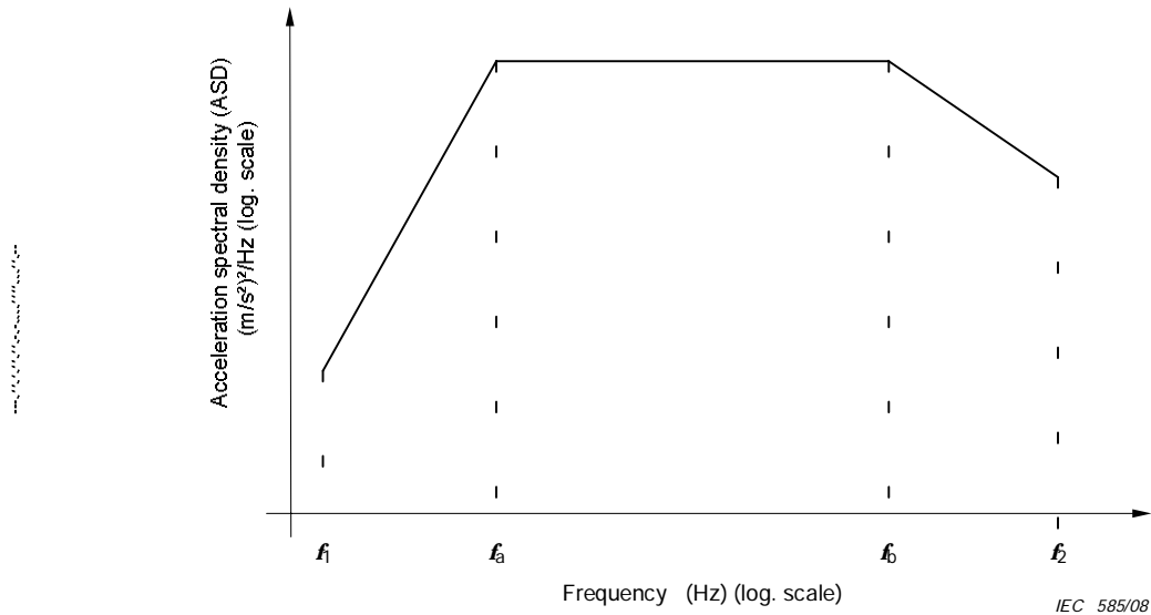
Figure A.3 – Equipment in wheeled vehicles – Frequency/amplitude break points
