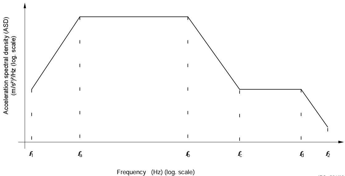
Figure A.4 – Equipment installed in airplanes and helicopters
