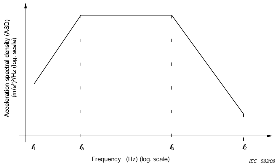
Figure A.1 – Frequency/amplitude break points – Transportation
